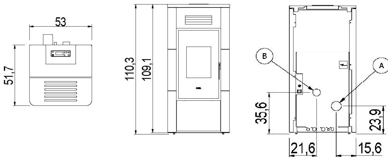
Fig. 20 - RIVER IDRO 18 - 24 ACL
