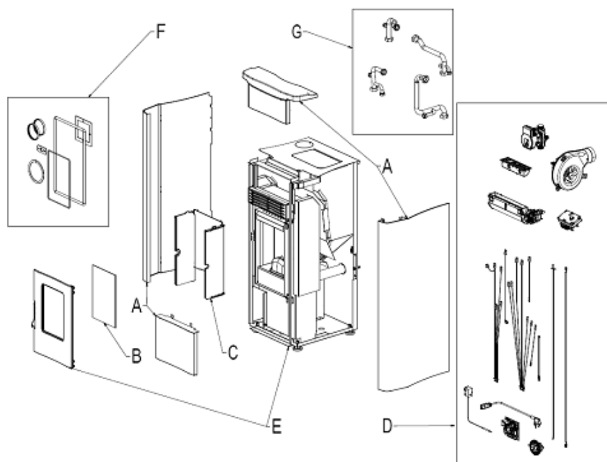
Fig. 1 - Exploded drawing
