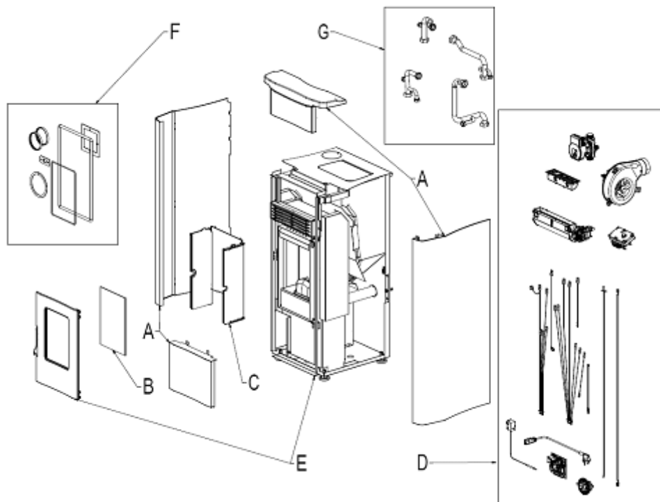
Fig. 1 - Exploded drawing
