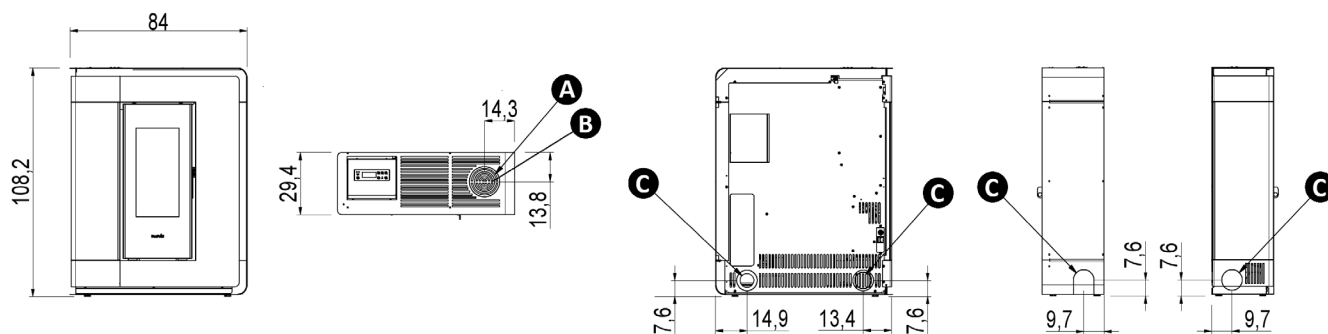
Fig. 26 - Arco 7/9 Bi-Flux
