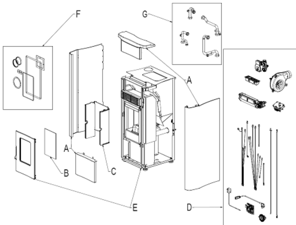
Fig. 1 - Exploded drawing
