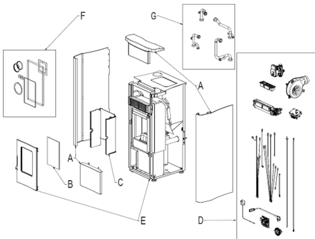
Fig. 1 - Exploded drawing
