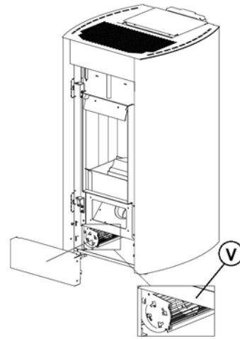
Fig. 91 - Ventilators
